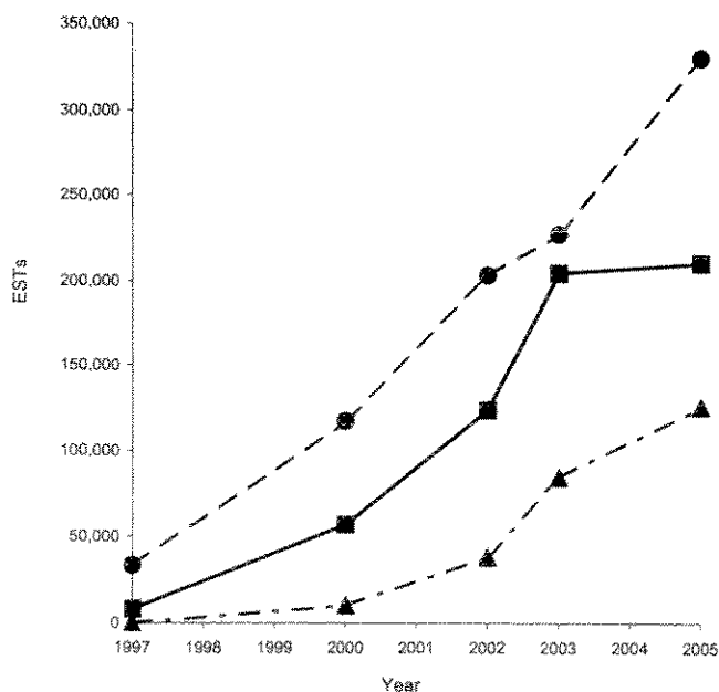
FIG. 1. EST generation from free-living nematodes including Caenorhabditis elegans (circles), mammalian parasitic nematodes (squares), and plant-parasitic nematodes (triangles) from 1997 to 2005. During that same time period, total nematode ESTs increased from 41,000 to 665,000 and total ESTs for all species increased from 872,000 to 28,800,000 (www.ncbi.nlm.nih.gov/dbEST/dbEST_summary.html).
